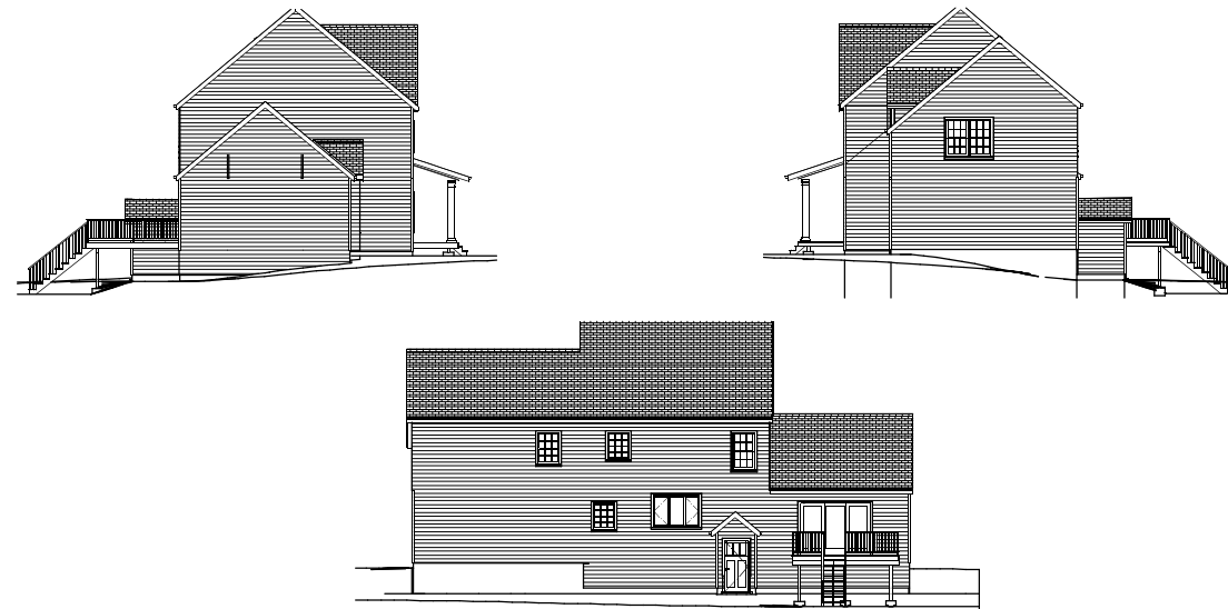
ALTERNATE ELEVATIONS
